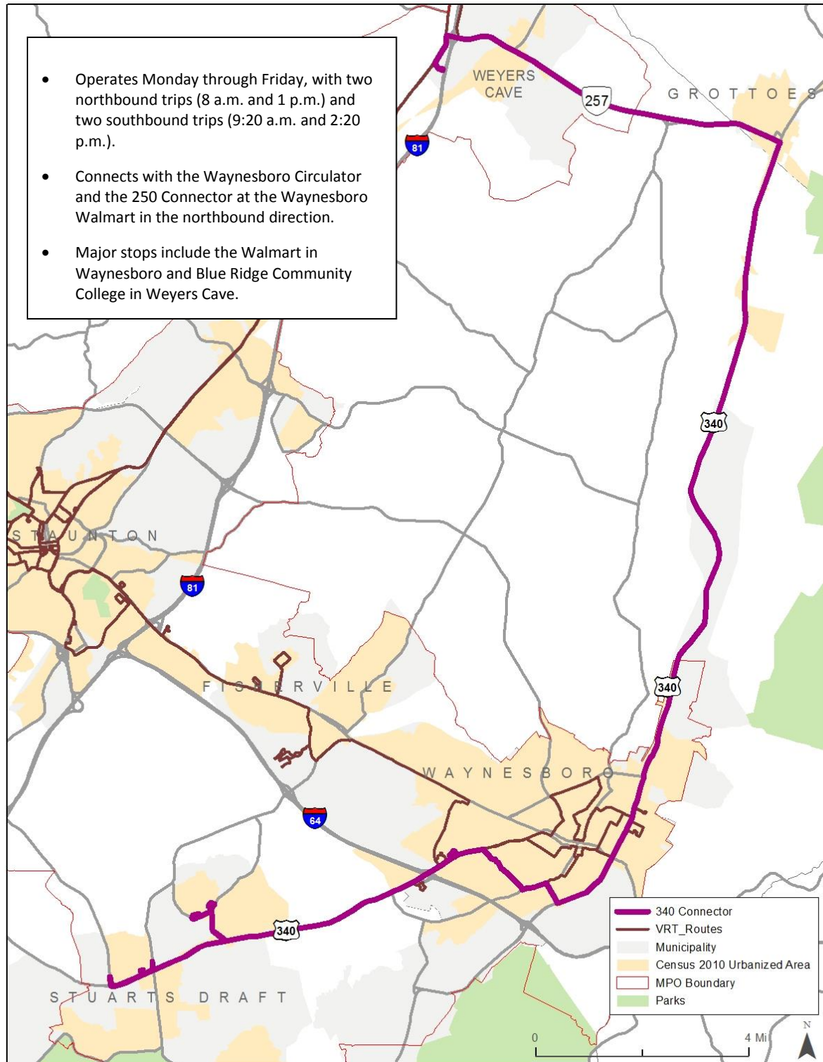
Figure 1-5: 340 Connector
